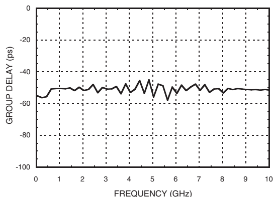
Group Delay
