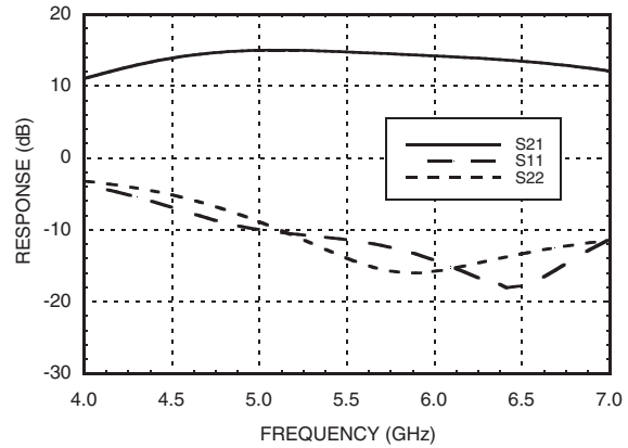
LNA Broadband Gain & Return Loss @ Vdd= 5V
