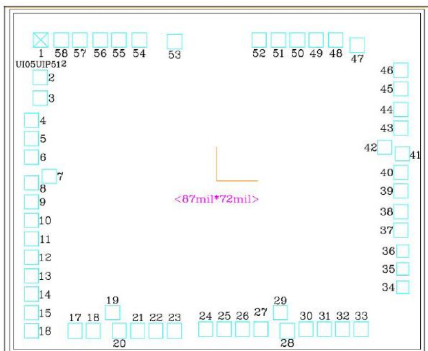
衬底面积:2205um*1815um(衬底接地)
