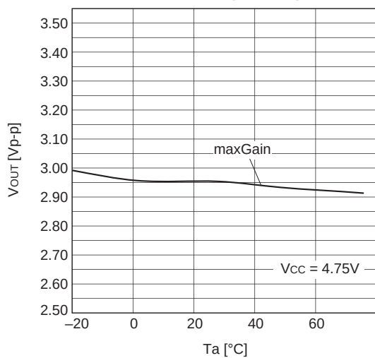
CL mode maximum signal amplitude temperature characteristics
