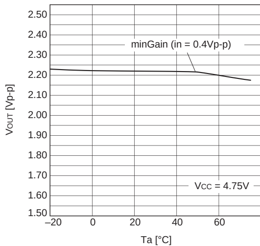
CAM mode maximum signal amplitude temperature characteristics
