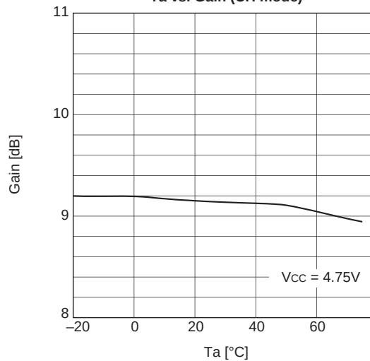
CH mode AMP gain temperature characteristics
