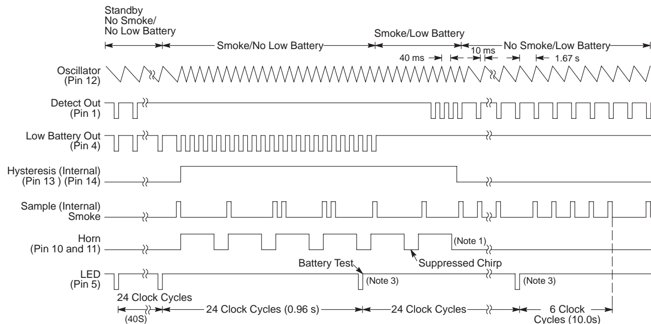
Figure 6. Timing Diagram
