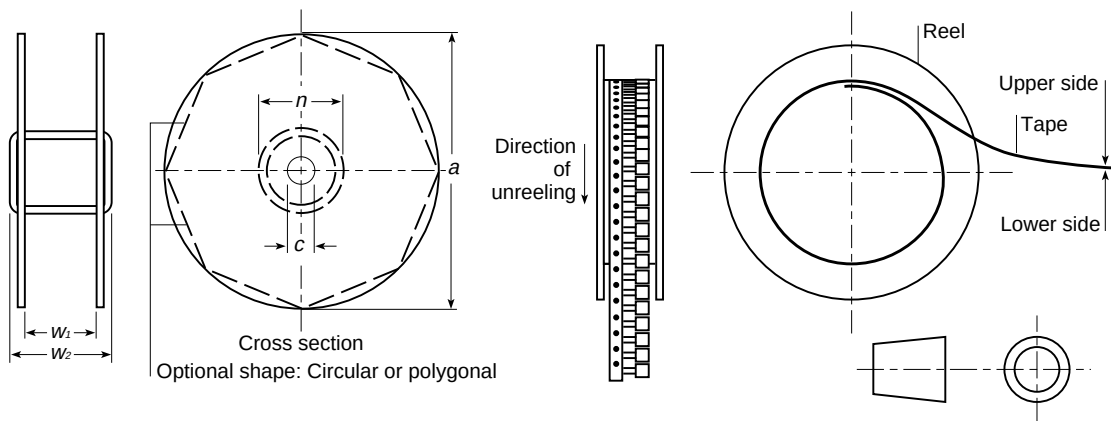
Figure R23. EIA Referenced Reel Dimensions for Radial-leaded Devices
