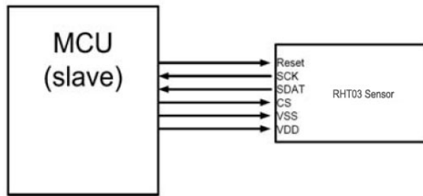
Figure 1: Typical Application
