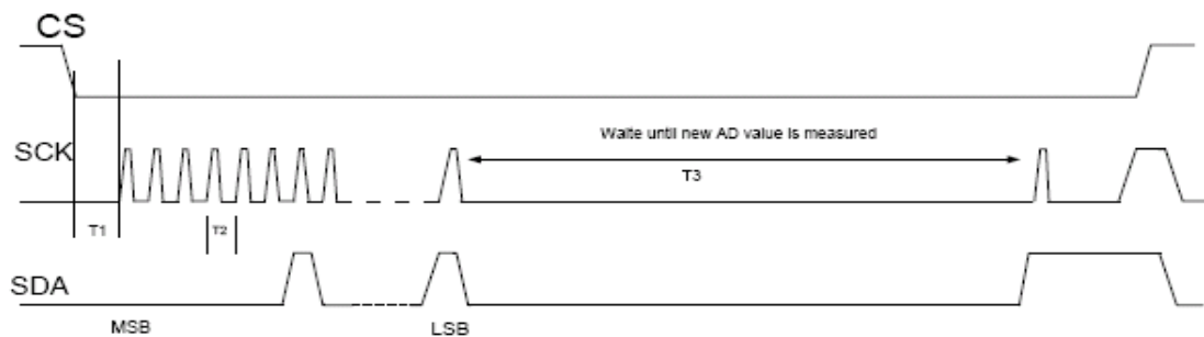
Figure 3: Bus timing
