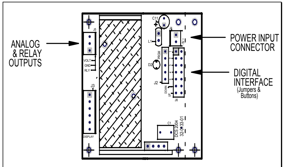
Figure 2: Model 305e Parts Locations.
