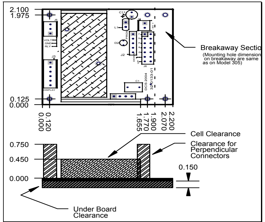
Figure 1: Model 305e Mechanical Dimensions.
