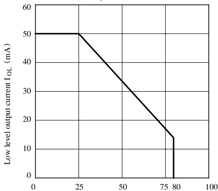
Fig. 1 Low Level Output Current vs. Ambient Temperature
