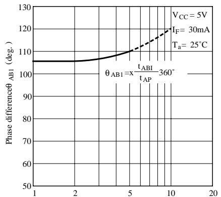
Fig. 4 Phase Difference vs. Frequency
