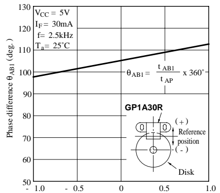
Fig.10 Phase Difference vs. Distance (Y direction)
