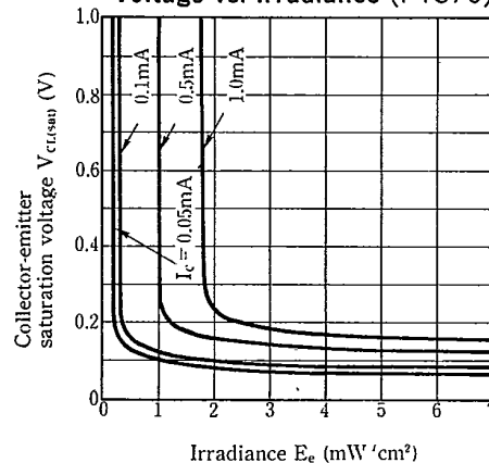
Fig. 19 Collector-emitter Saturation Voltage vs. Irradiance (PT372)
