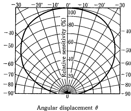
Fig. 15 Sensitivity Diagram (PT371) ( T_a = 25^\circ\text{C} )
