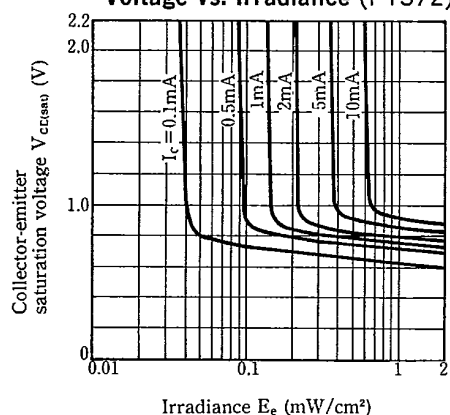
Fig. 19 Collector-emitter Saturation Voltage vs. Irradiance (PT372)
