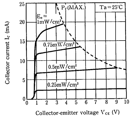
Fig. 10 Collector Current vs. Collector-emitter Voltage (PT372)
