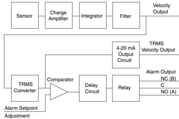
K-Guard Block Diagram
