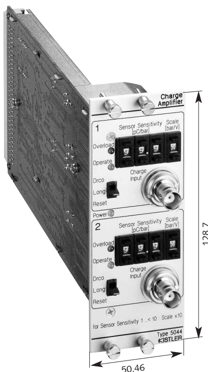
Fig. 2: Charge amplifier Type 5044A
