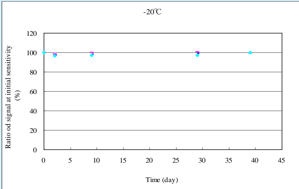
Fig.8: Durability in low temperature (-20°C)
