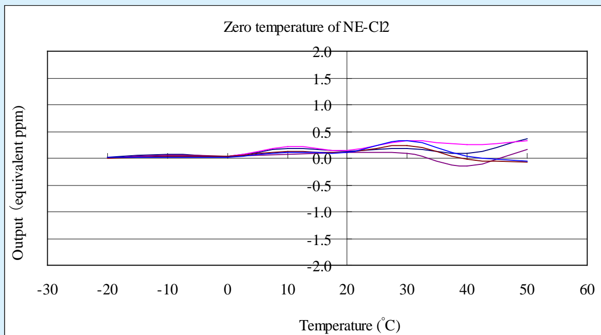
Fig. 3 : Typical temperature coefficient of NE4-CI2 (100 at 20 °C)
