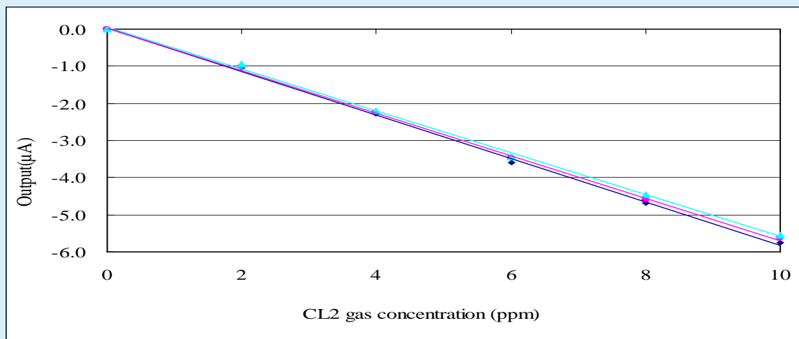
Fig.2: Gas Sensitivity of NE4-Cl2
