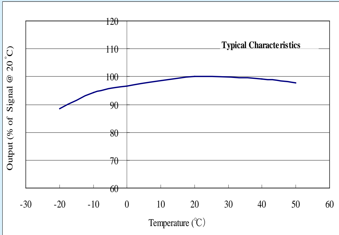
Fig. 4: Typical temperature coefficient of NE4-Cl2 (100 at 20 °C)
