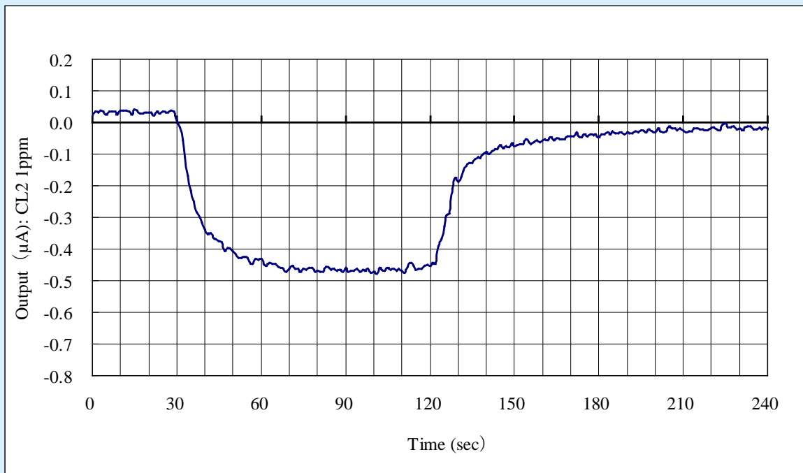
Fig.5: Response and recovery characteristics of NE4-Cl2 (at 20 °C)
