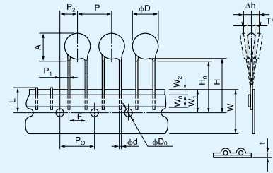
Straight Leads and Taped Z7D □□□ T4D
