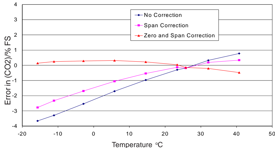
Figure 4 Temperature Compensation
