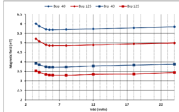
11.2 Magnetic parameters vs. V_{DD}
