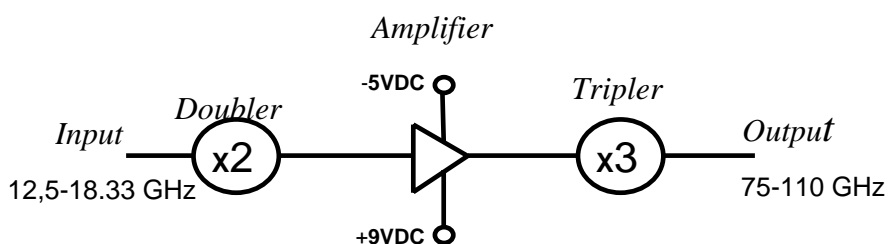
Schematic diagram of BFM-10/6
