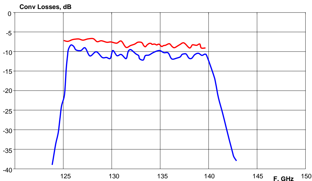
Conversion Losses of the Downconverter Flo= 121.4GHZ RF=127.4-139.4GHz
