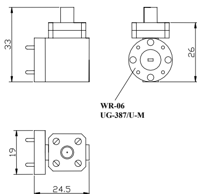
Outline drawing of ZBD-06 detector
