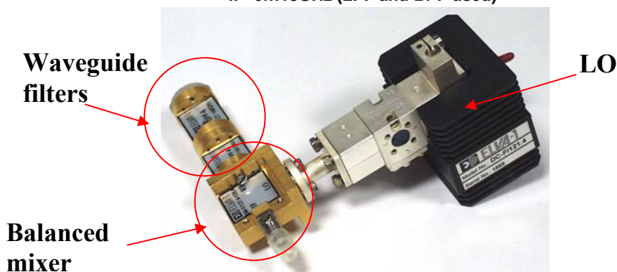
F-band Downconverter LO= 121.4GHz RF=127.4-139.4GHz IF=6...18GHz (LPF and BPF used)
