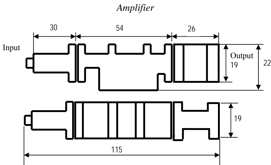
Outline drawing of BFM-10/6 multiplier (mm)
