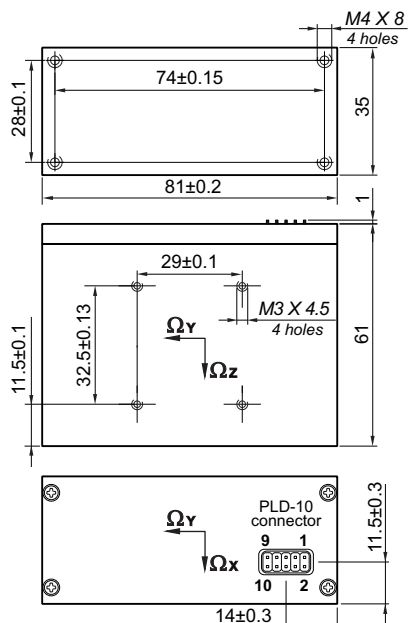
OUTLINE DRAWING
